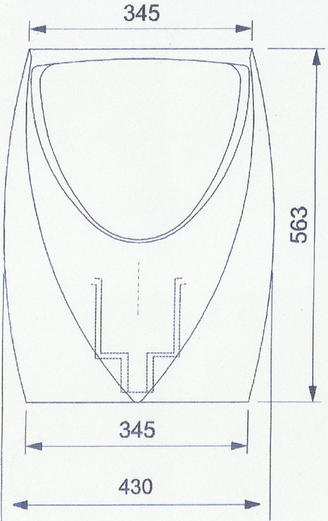
Dimensions are in mm
